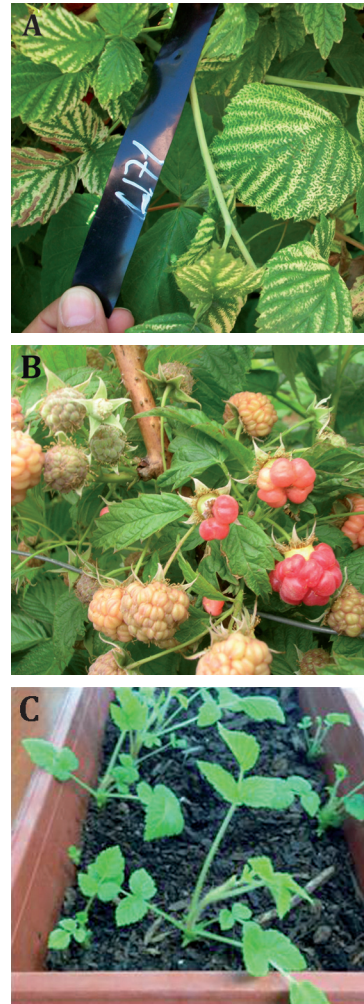
Figure 1. Symptoms ToRSV in raspberry leaves and fruits. Yellowing presence of primary and secondary veins in 3 and 12 year old plants of the Meeker (1A) and Heritage (1B) varieties. 1C, regrowth asymptomatic plant of 5 year old, variety Meeker.
